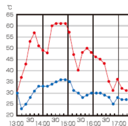
Coolbit Water Injection Cap Cooling Effect Graph
